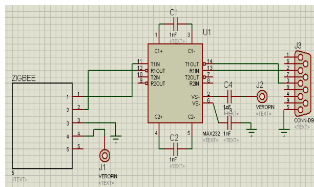
Fig. 4. Transmitter circuit diagram
