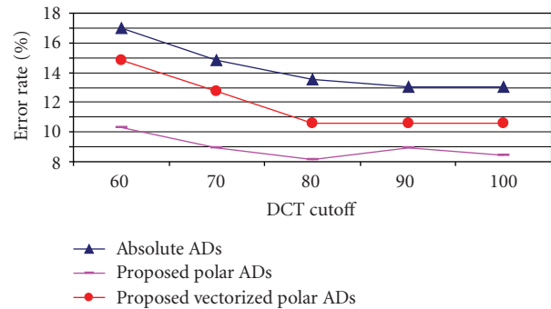
FIGURE 12: Fisher’s linear discrimination with vertical Radon transformation and ideal lowpass filtering.
