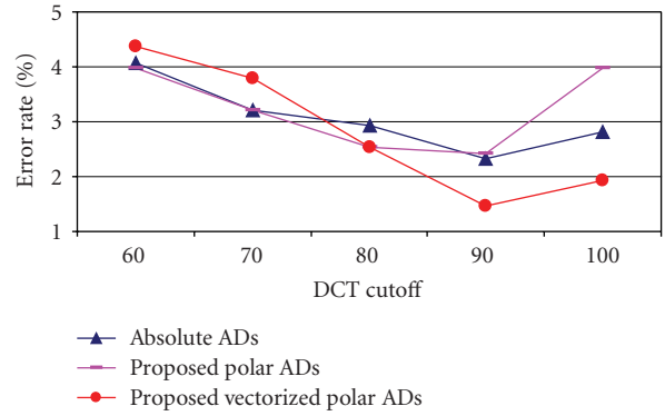
FIGURE 11: Fisher’s linear discrimination with 2D transformation and zonal coding.
