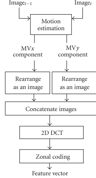
FIGURE 1: Block diagram of time-dependent feature extraction from motion vectors.
