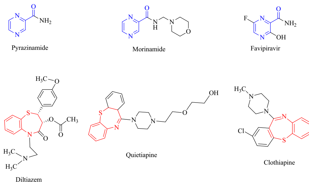
Fig. 1 Representative structures of clinically used pyrazine and benzothiazepine ring containing drugs.
