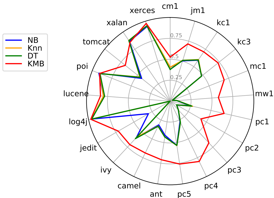
Figure 5. Precision for the basic classifiers and KMB.
