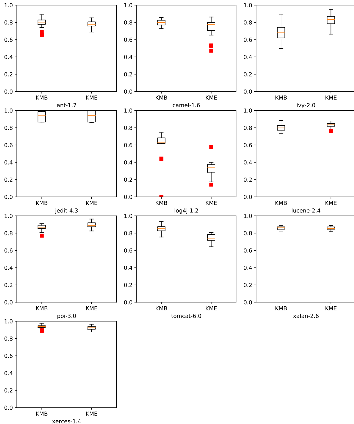
Figure 12. Boxplot representing the G-mean of KMB and KME for PROMISE datasets.
