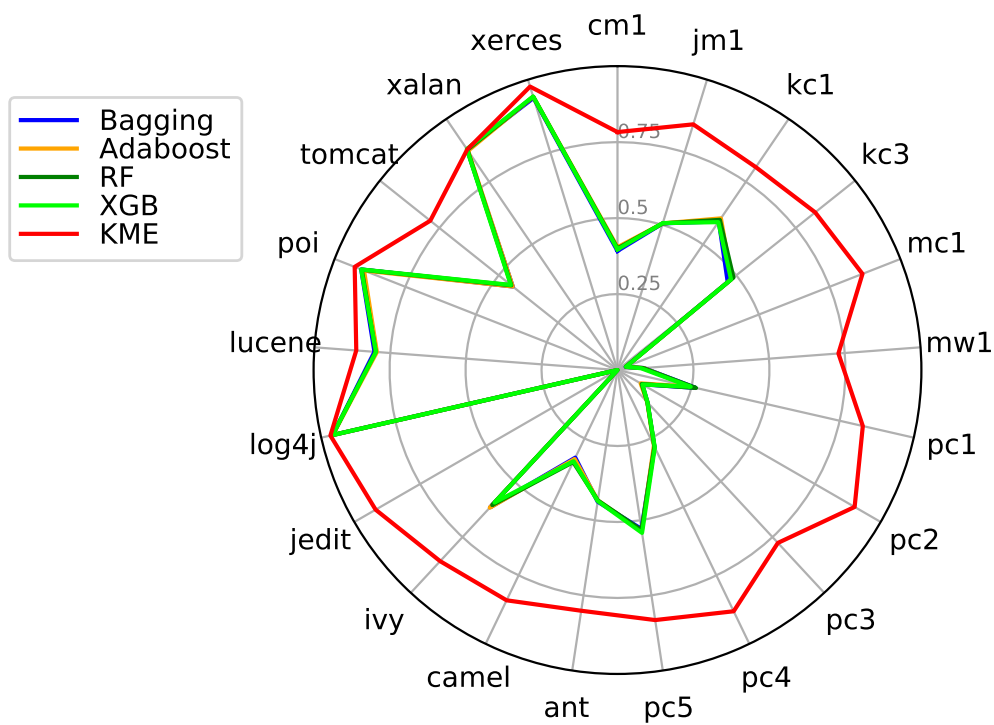
Figure 8. Precision for the ensemble classifiers and KME.
