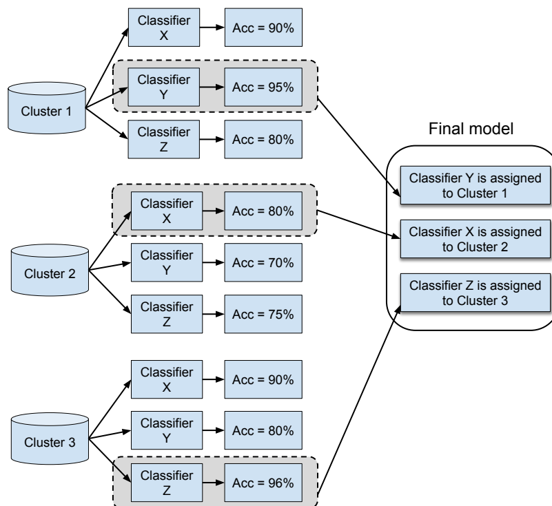
Figure 2. Example of the model development phase of the proposed approach.
