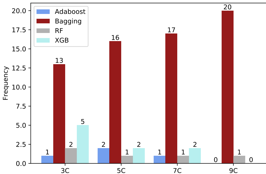
Figure 4. Frequency of the ensemble classifiers in K-Means/Ensemble classifiers (KME) for different numbers of clusters.
