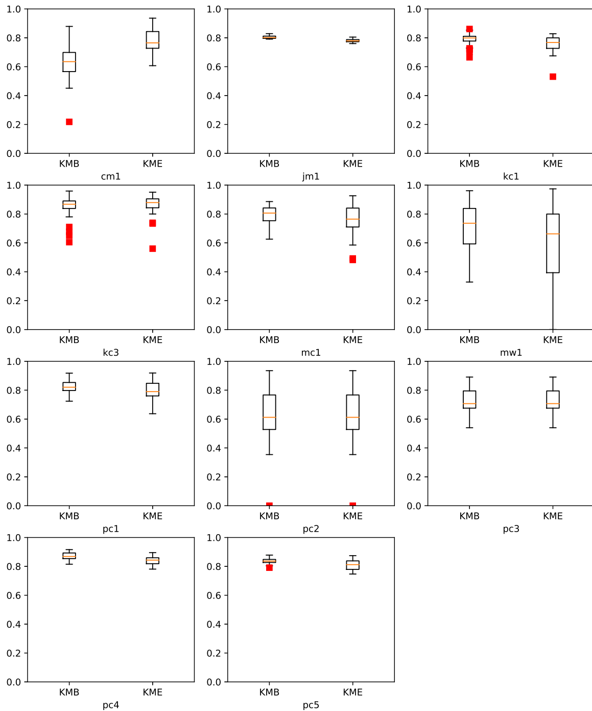
Figure 11. Boxplot representing the G-mean of KMB and KME for NASA datasets.
