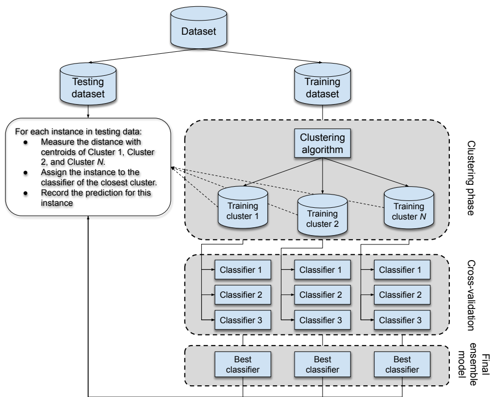
Figure 1. Proposed methodology for software defect prediction.
