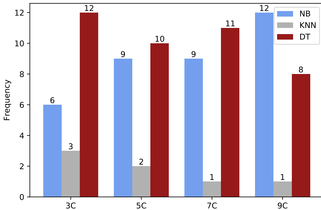
Figure 3. Frequency of the basic classifiers in K-Means/Basic classifiers (KMB) for different numbers of clusters.
