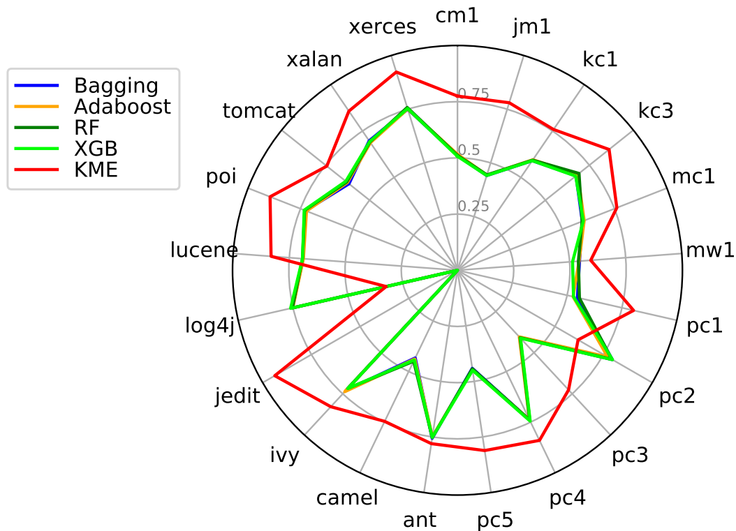
Figure 10. G-mean for the ensemble classifiers and KME.
