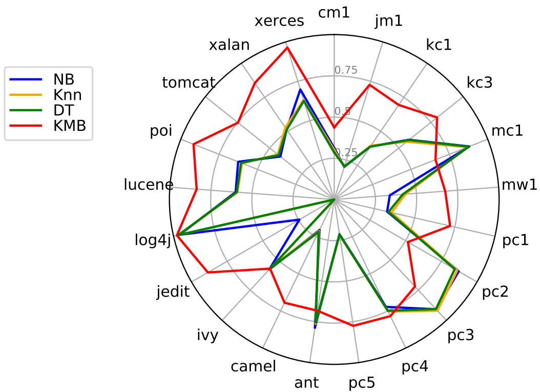
Figure 6. Recall for the basic classifiers and KMB.
