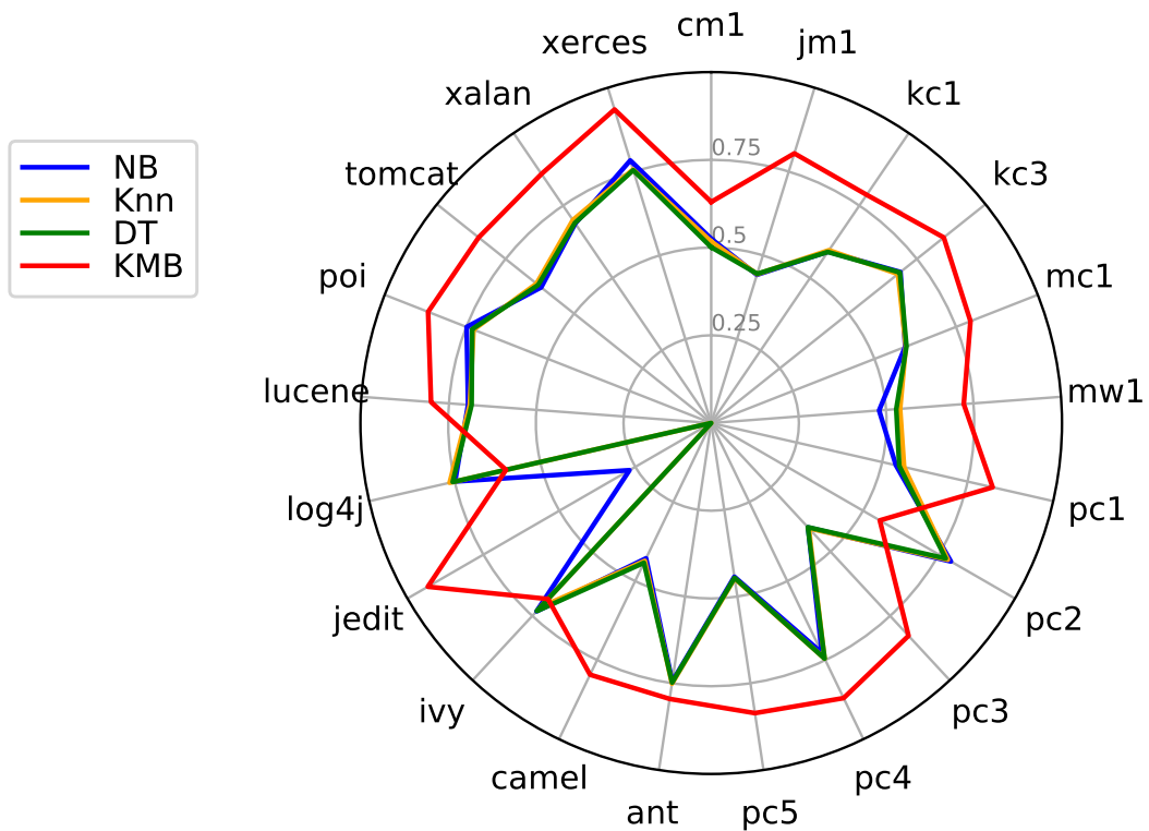
Figure 7. G-mean for the basic classifiers and KMB.
