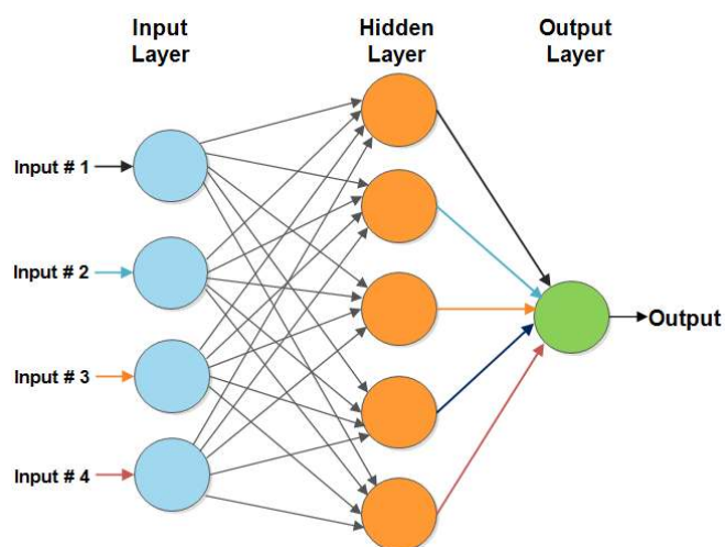
Figure 2. Multilayer Perceptron.
