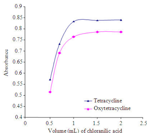
Fig. 2: The effect of chloranilic acid volume on the charge complex reaction with tetracyclines
