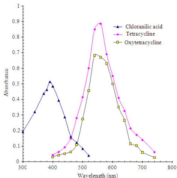
Fig. 1: Absorption spectra of the products of tetracycline ( 30 \mu\text{g mL}^{-1} ) oxytetracycline ( 15 \mu\text{g mL}^{-1} ) and p chloranilic acid
