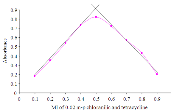
Fig. 3: The continuous variation method for the stoichiometry of the reaction of chloranilic acid and tetracycline
