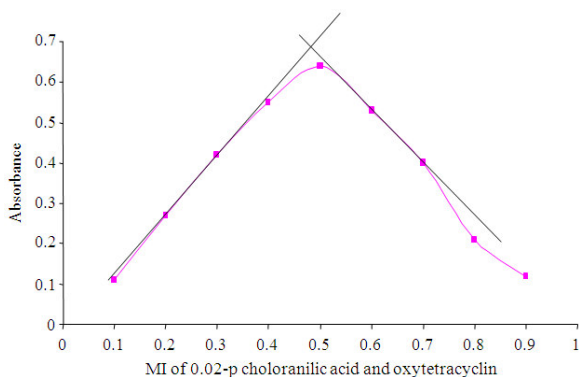
Fig. 4: The continuous variation method for the stoichiometry of the reaction of chloranilic acid and oxytetracycline
