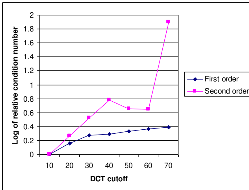
Figure 6. Log of relative condition number of matrix \mathbf{R} in Equation 10 for 1 st and 2 nd order polynomial expansions.
