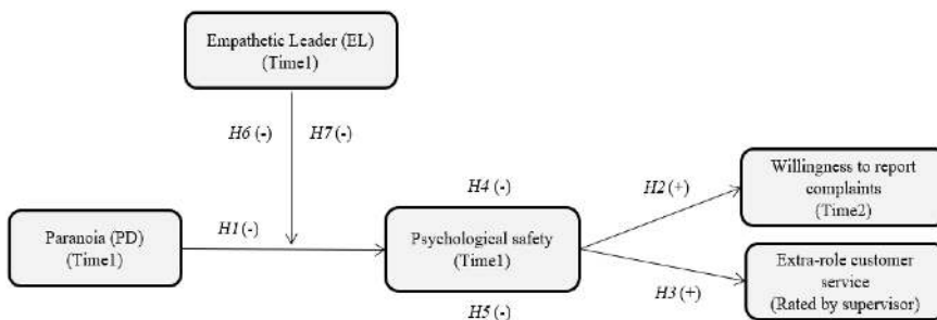
Figure 1. Hypothesized model
