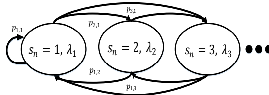
Figure 5. Markov Modulated Poisson Process model used in [22]. s_n represent the number of M2MD transmitting data and \lambda represent the state arrival rate.
